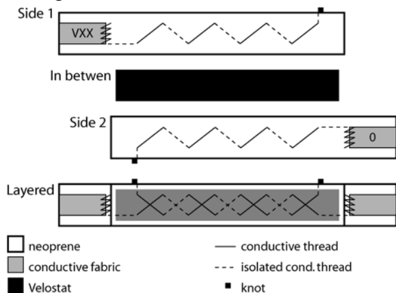
Fig 1. Bend Sensor, construction (15 mm width)
