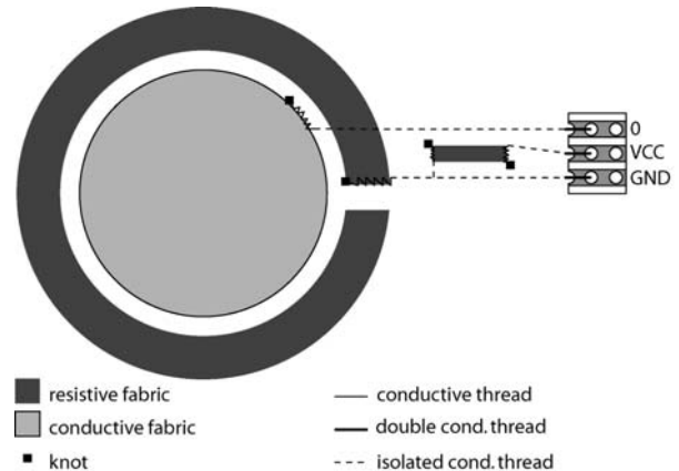
Figure 4. Fabric Potentiometer
